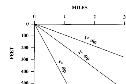
FIGURE 6. The above diagram illustrates the conversion of apparent dip to true dip. One is provided on each page of cross sections. The dip conversion diagram is designed to give the user a mental picture of the relief distortion that is caused by the vertical exaggeration.
